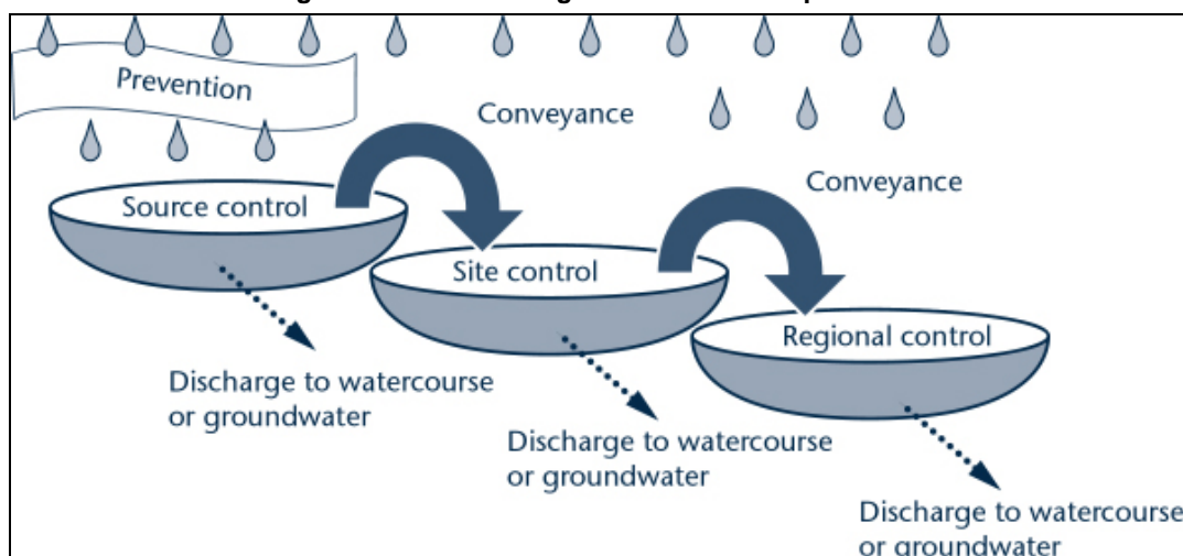
Figure D1: SuDS Management Train Principle 12
